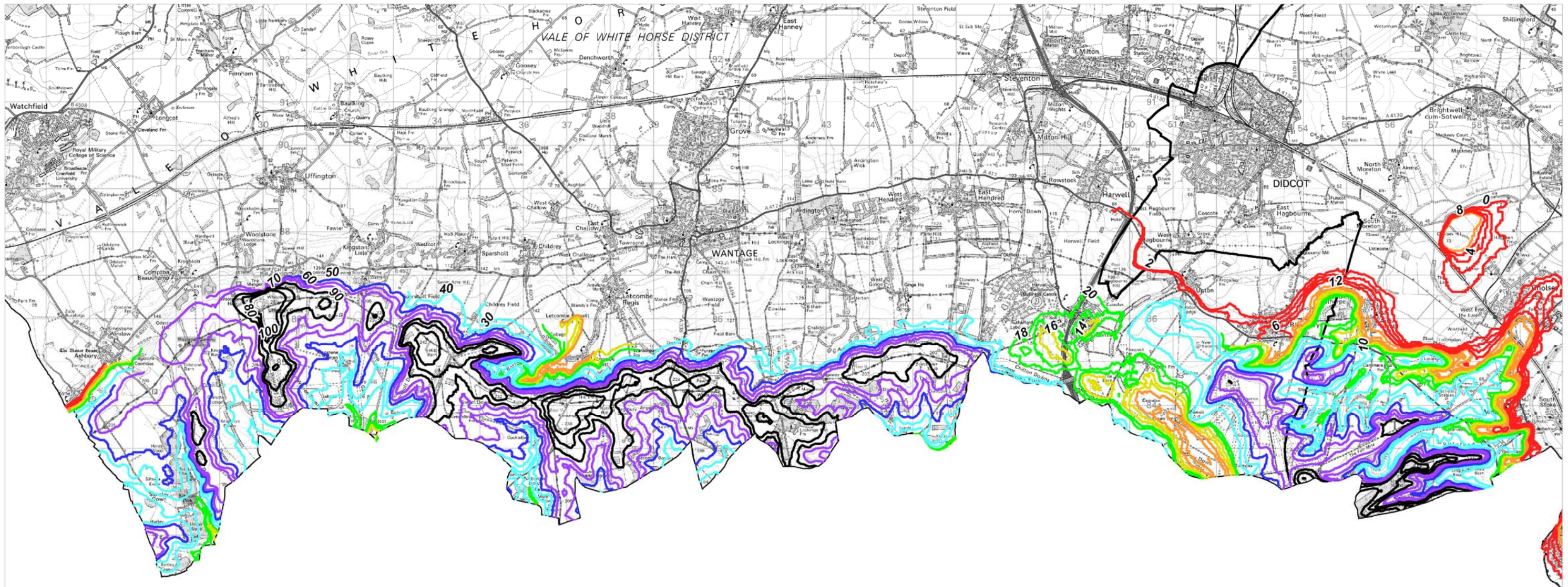
Figure E-16: Groundwater Depth (m)
